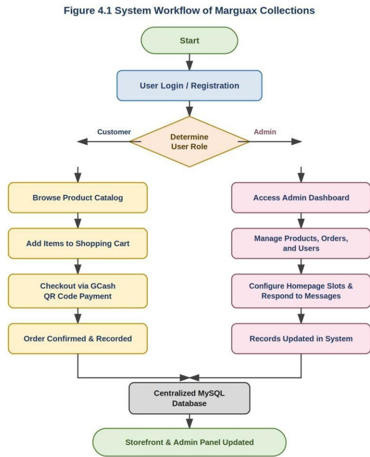
Figure 4.1. System Workflow of Margaux Collections
