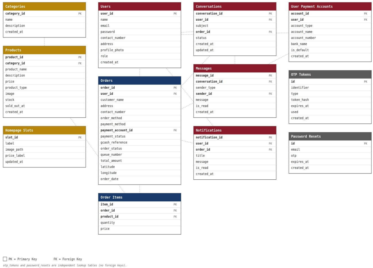
Figure 4.4. Entity Relationship Diagram of Margaux Collections
